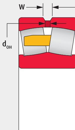
Dimensions of Oil Grooves and Holes (mm)
